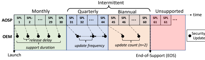
Fig. 2: A representative illustration of the support lifecycle of an Android device.
